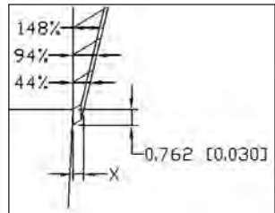
Double Hollow Bevel
