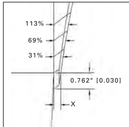
DOUBLE HOLLOW BEVEL
