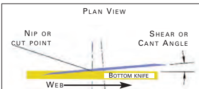
Shear Angle Geometry
