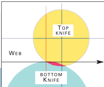
• Cut Point
