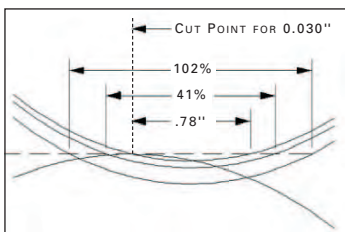
CHORD FOR A 6" O.D. blade
